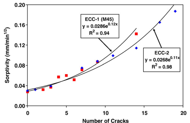
Fig. 8. Sorptivity versus number of crack.
