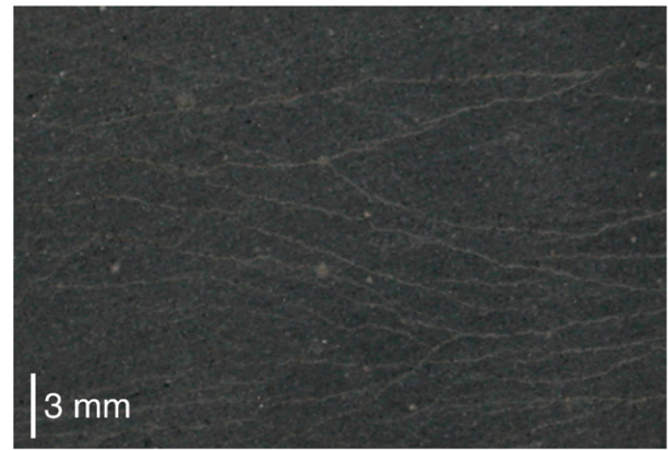
Fig. 2. Typical crack pattern on positive moment surface of ECC beams at 2 mm deformation [5].
